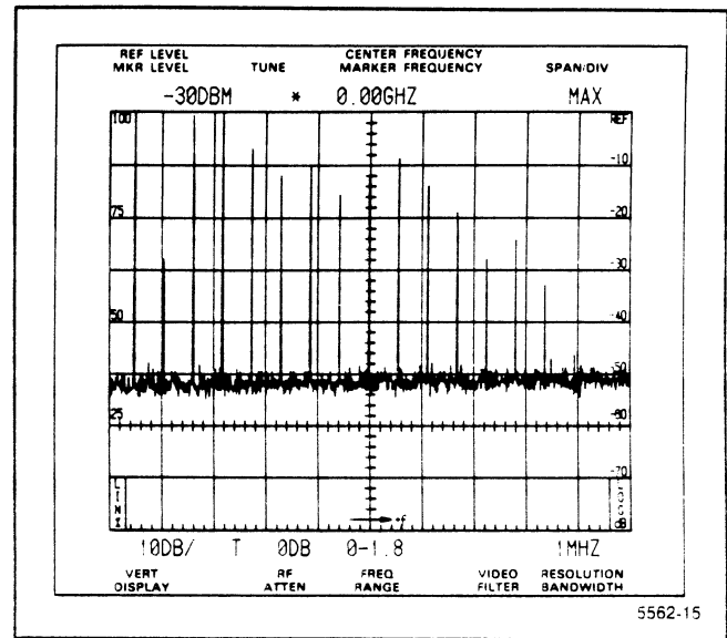
Figure 5-2. Typical display of calibration markers in the maximum span position.
